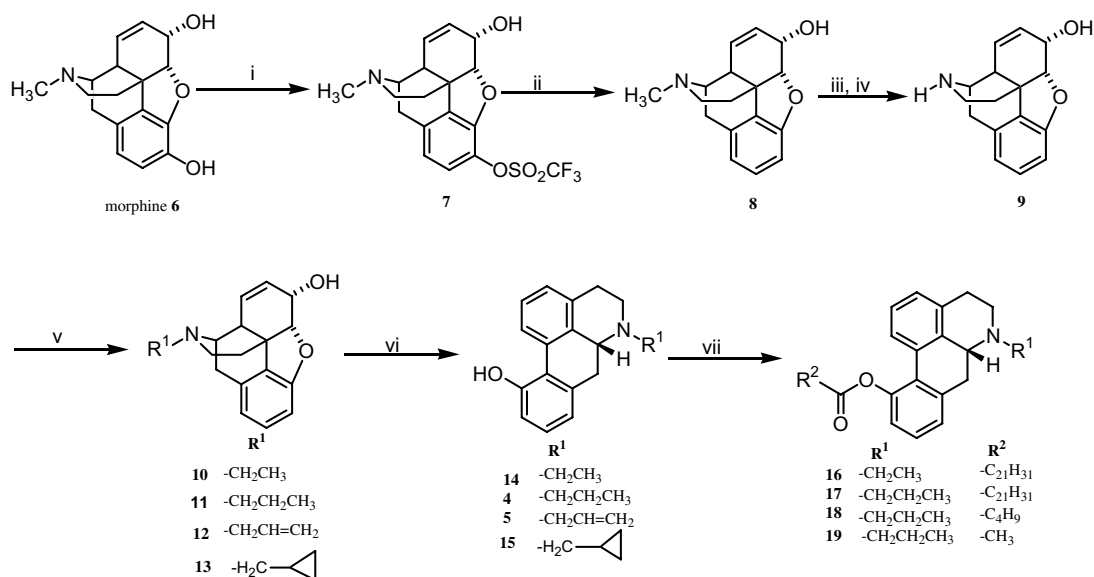
Scheme 1. Synthesis of N -alkylated-11-hydroxynoraporphines and their esters. Reagents and conditions: (i) PhNTf 2 , Et 3 N, CH 2 Cl 2 , overnight; (ii) Pd(OAc) 2 , Ph 3 P, Et 3 N, HCOOH, DMF, 60 °C; (iii) ClCOOCH 3 , NaHCO 3 ; (iv) NH 2 NH 2 , reflux; (v) R 1 X, K 2 CO 3 , EtOH; (vi) CH 3 SO 3 H; (vii) R 2 COOH, DCC, DMAP, CH 2 Cl 2 .
